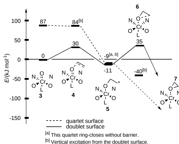
Figure 2. The PES at the B3LYP/BSII/B3LYP/BSI level for systems b .
