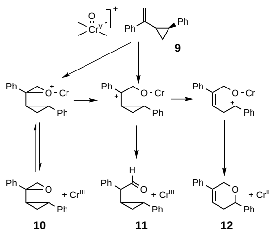
Scheme 4. Possible pathways for the formation of 10 – 12 .
