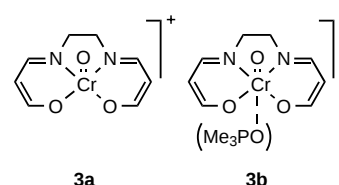
Scheme 1. Truncated molecules used in the calculations. Species without donor ligand are denoted a ; with donor b .
