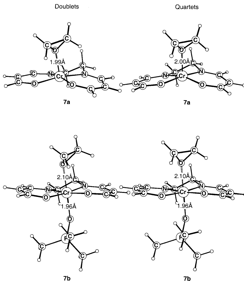
Figure 7. Product complexes 7a and 7b .
