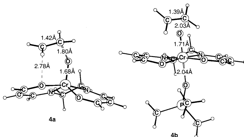
Figure 4. Transition states 4a and 4b in the doublet states.
