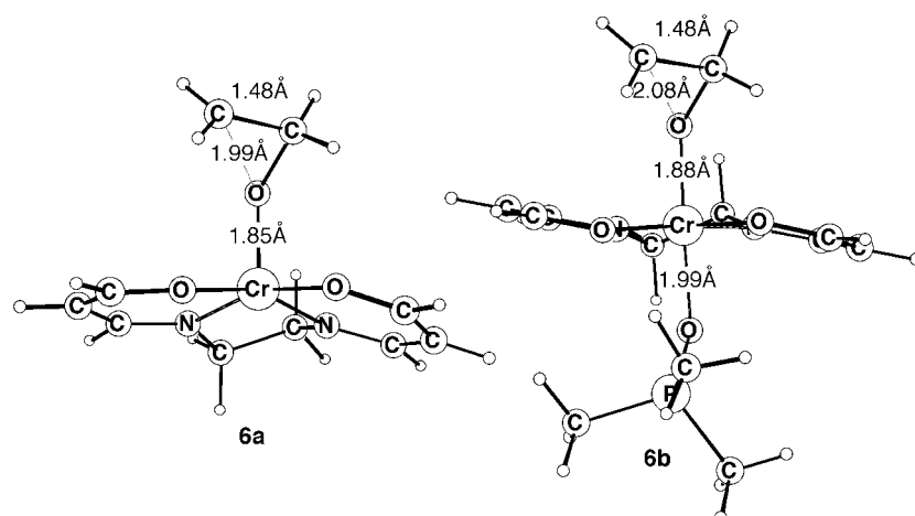
Figure 6. Transition states 6a and 6b for ring closure of the intermediate ethyl radicals (doublets).
