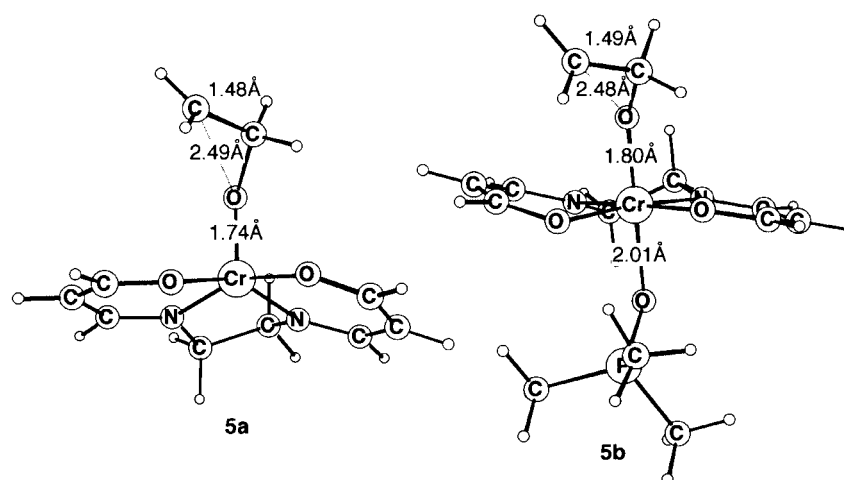
Figure 5. Intermediate ethyl radicals 5a and 5b .
