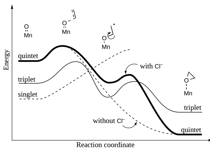
Figure 1. Qualitative consensus PES for the reaction of (salen)Mn=O species with alkene, collected from literature sources. [7, 9, 10]
