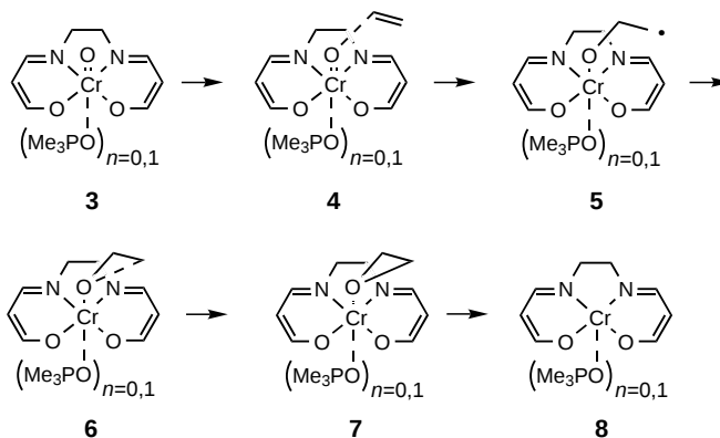
Scheme 2. Species evaluated in the quantum chemical study ( a : n=0 ; b : n=1 ).
