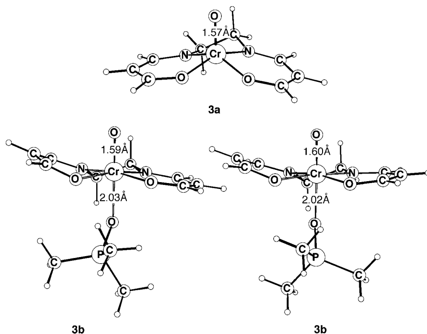
Figure 3. Structures of the doublet Cr oxo complexes 3a and 3b .
